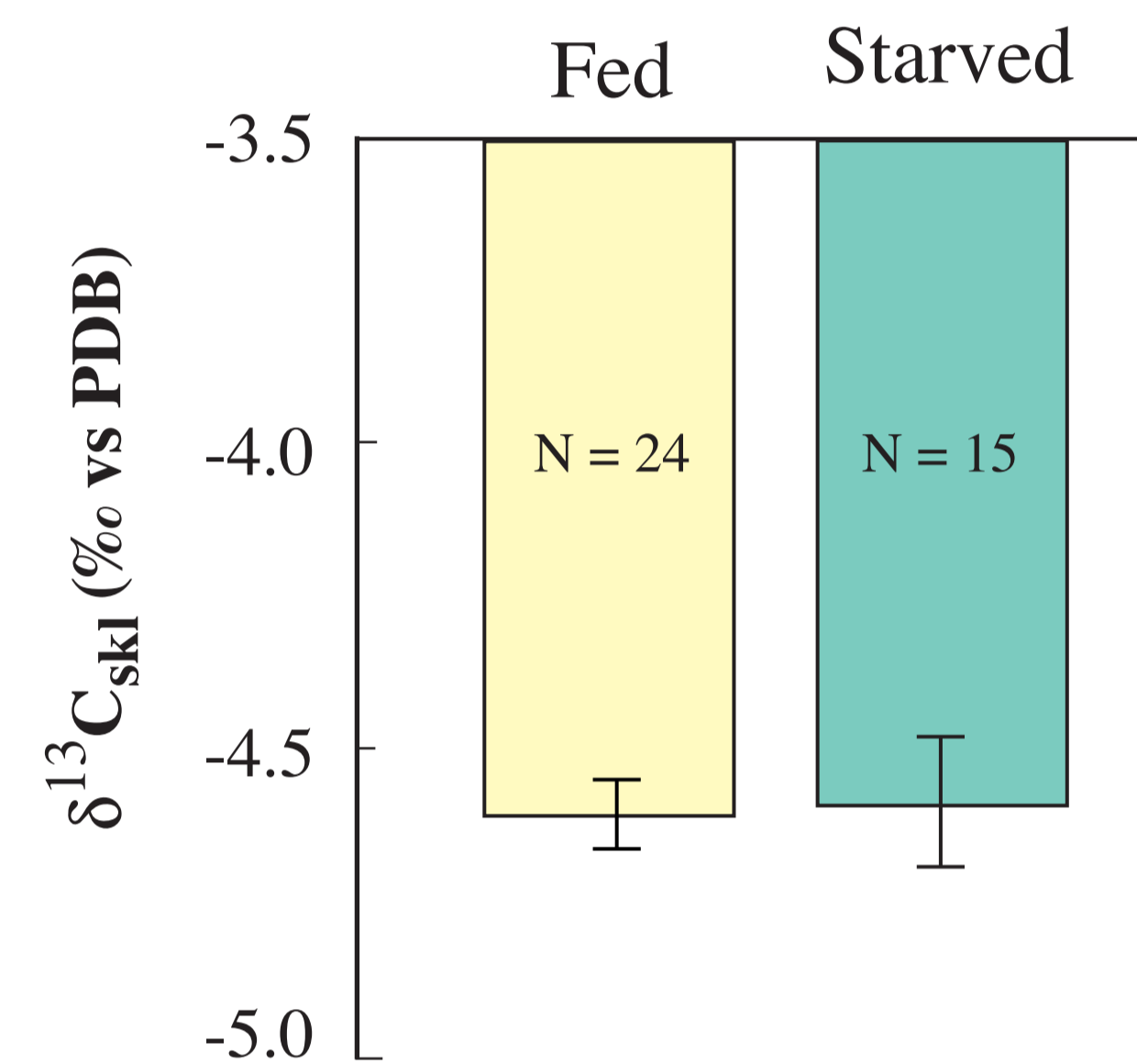
Skeletal \delta^{13}\text{C} in fed and starved colonies of Stylophora pistillata . Mean \pm standard error of the mean.
