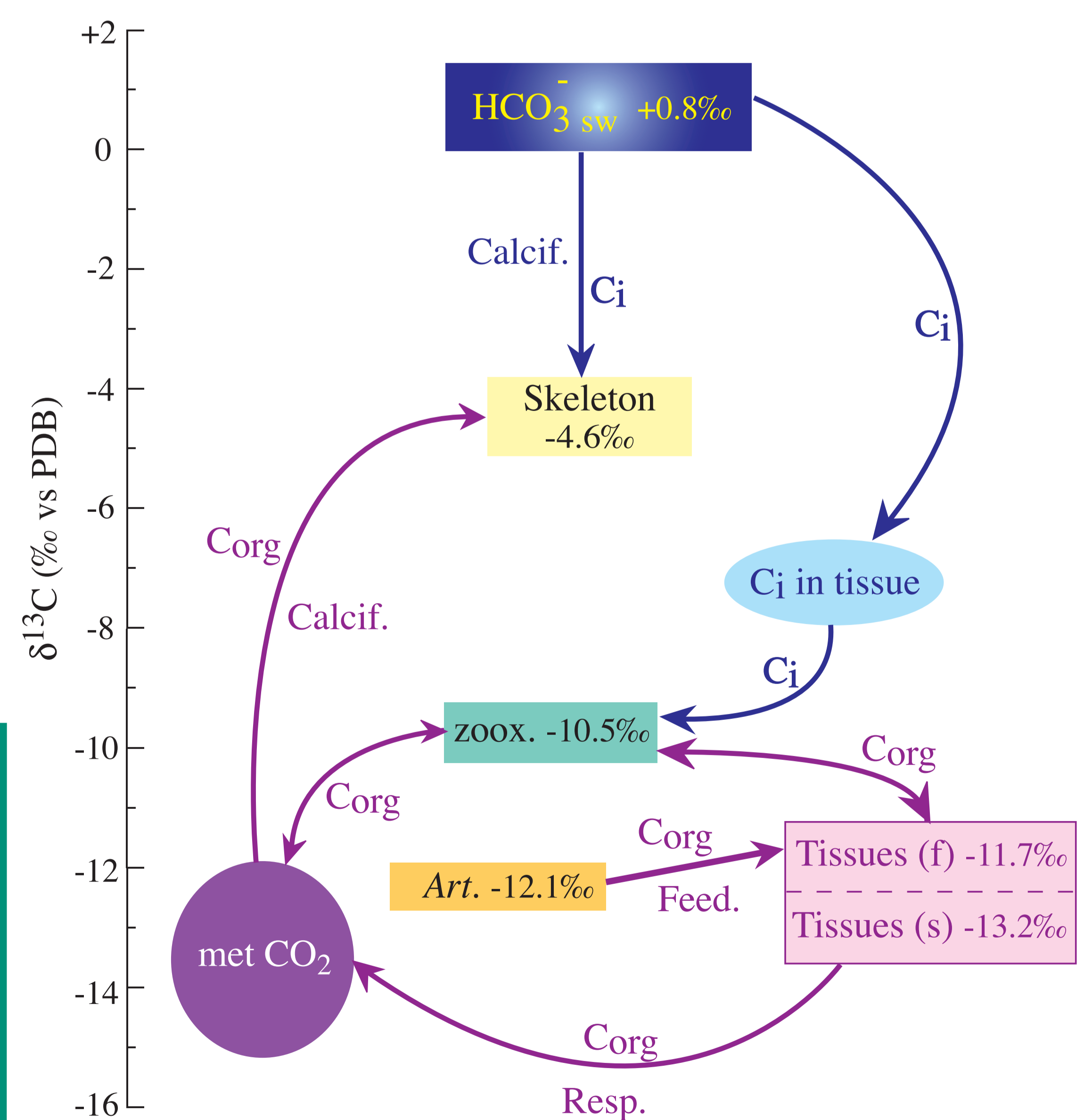
Model of carbon flow among several compartments in Stylophora pistillata . Square boxes represent measured pools, whereas circles represent inferred isotopic values. (Ci: inorganic carbon, Corg: organic carbon, calcif.: calcification, resp.: respiration, feed.: feeding, zoox.: zooxanthellae, sw: seawater, Art.: Artemia , f: fed, s: starved, met.: metabolic).
