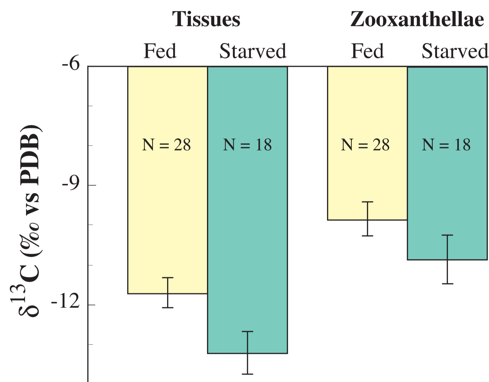
\delta^{13}\text{C} values of tissues and zooxanthellae for fed and starved colonies of Stylophora pistillata (mean \pm standard error of the mean).
