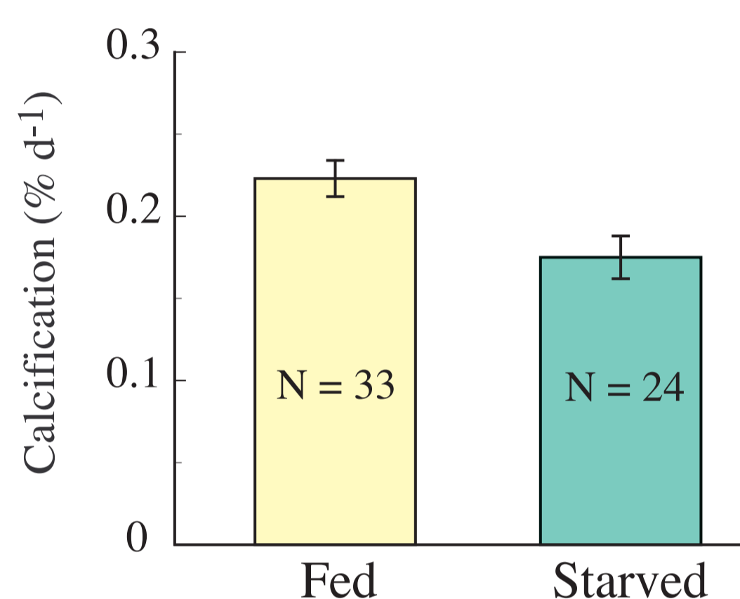
Calcification rate (% d -1 ) of Stylophora pistillata measured during 12 weeks of culture for fed and starved colonies. Mean \pm standard error of the mean.
